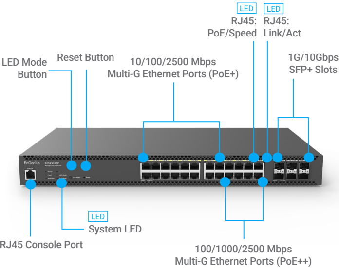
CloudSwitch MGPlus 24 Full PoE 6 SFP+ (ECS2530FP)
