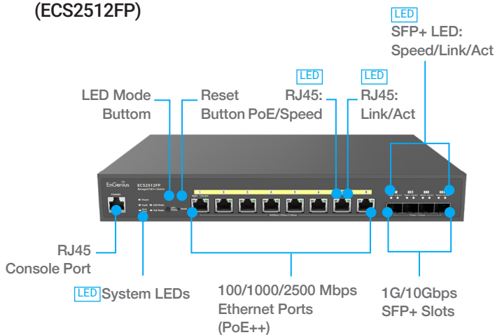
CloudSwitch MGPlus 8 Full PoE (ECS2512FP)
