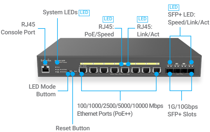
CloudSwitch Aggregate 8XG Full PoE (ECS5512FP)
