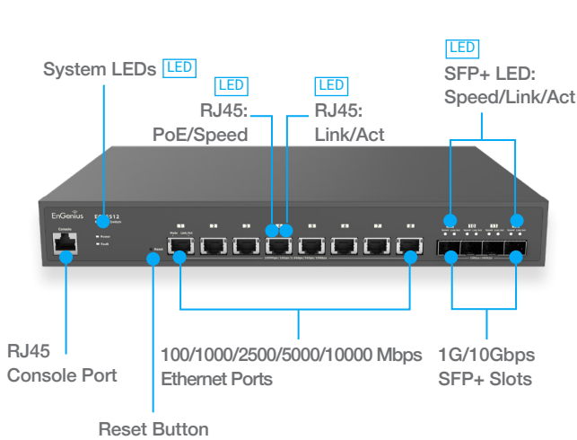
CloudSwitch Aggregate 8XG (ECS5512)
