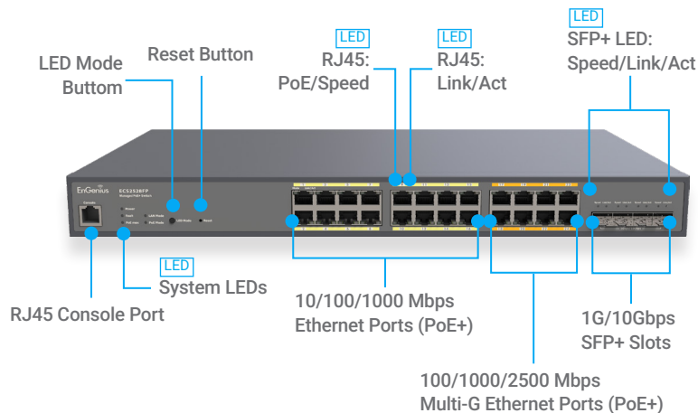
CloudSwitch MGPlus 24 Full PoE (ECS2528FP)
