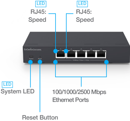
CloudSwitch MGLite 5 (ECS205L)
