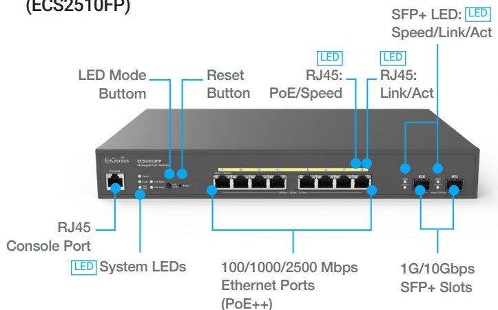
CloudSwitch MGPlus 8 Full PoE (ECS2510FP)
