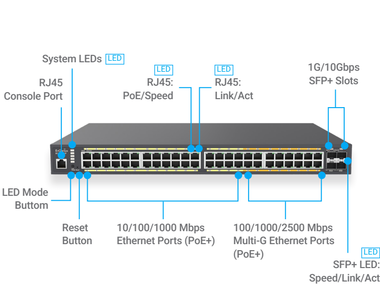
CloudSwitch MGPlus 48 Full PoE (ECS2552FP)
