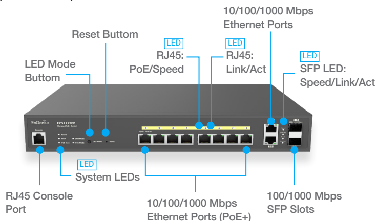
CloudSwitch L2Plus 8 Full PoE (ECS1112FP)
