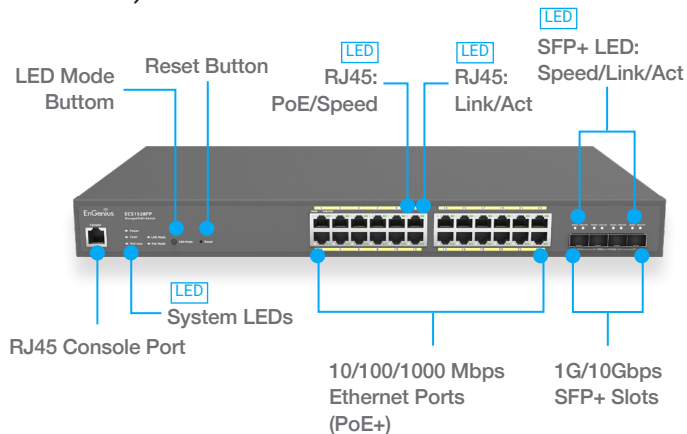
CloudSwitch L2Plus 24 Full PoE (ECS1528FP)
